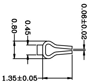
SEC:C-C
