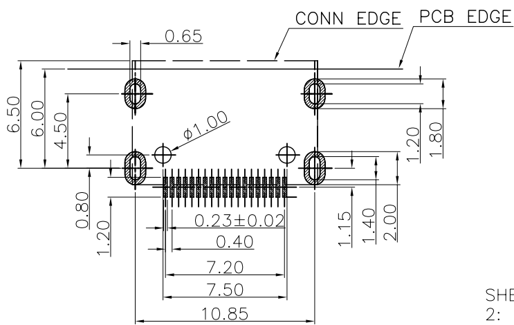
RECOMMENDED PCB LAYOUT(TOP VIEW) (THICKNESS=0.8±0.05mm) TOLERANCE = ±0.05
